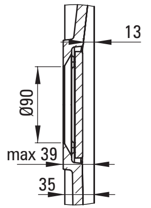
DETAIL B SCALE 1 : 3
